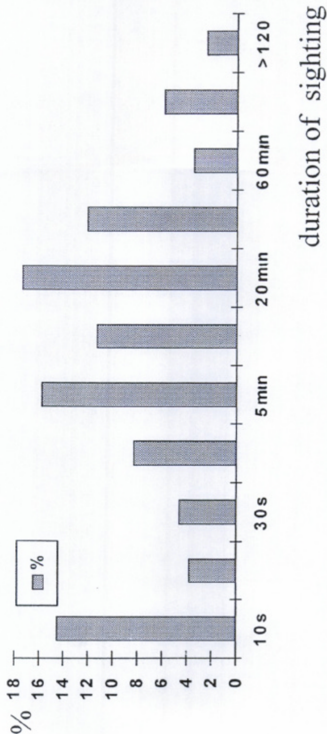
FIGURE 3-16 UAP EVENT DURATION 1996-1997
